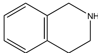
1,2,3,4-tetrahydroisoquinoline 91-21-4
