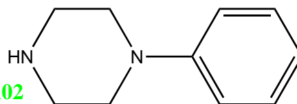
1-phenylpiperazine 2210-93-7
