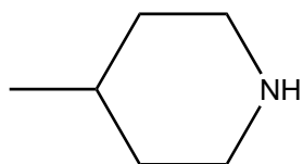
4-methylpiperidine 626-58-4
