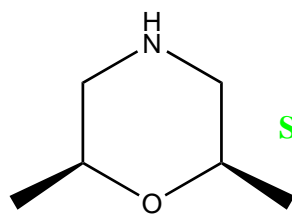
cis -2,6-dimethylmorpholine 6485-55-8
