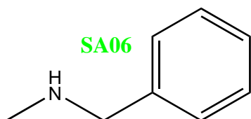
N -methyl(phenyl)methanamine 103-67-3
